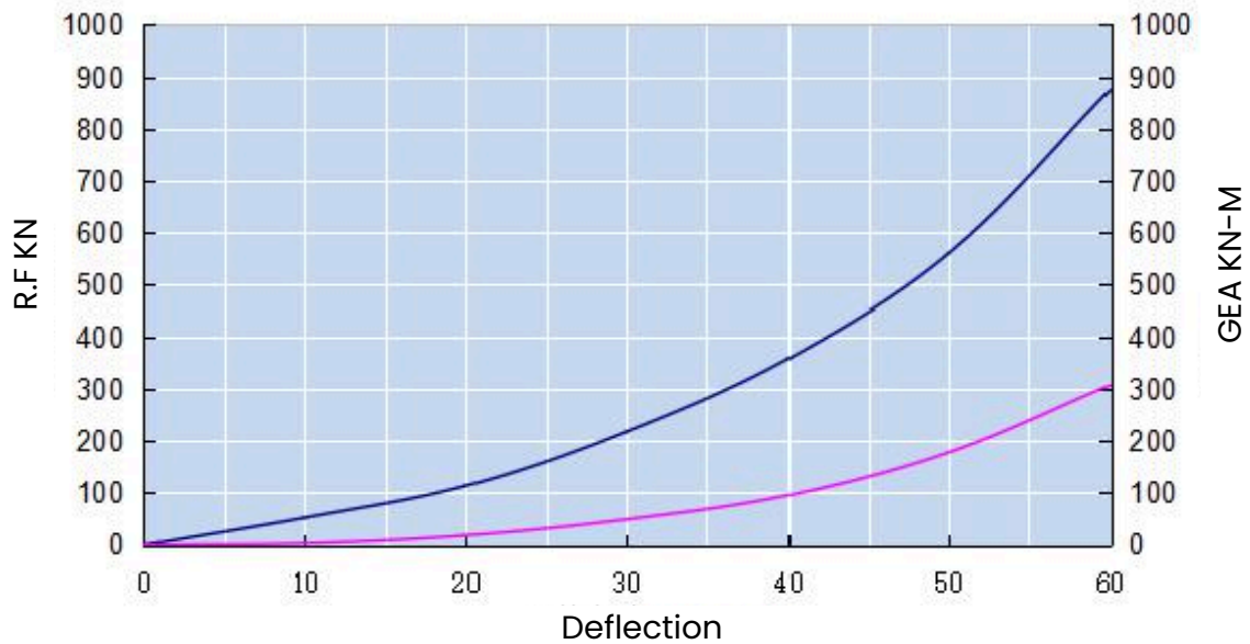
P50-2035/ Performance Curve
