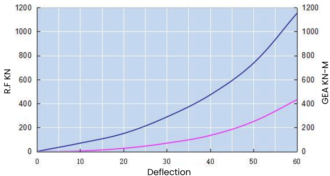
P80-2035/ Performance Curve
